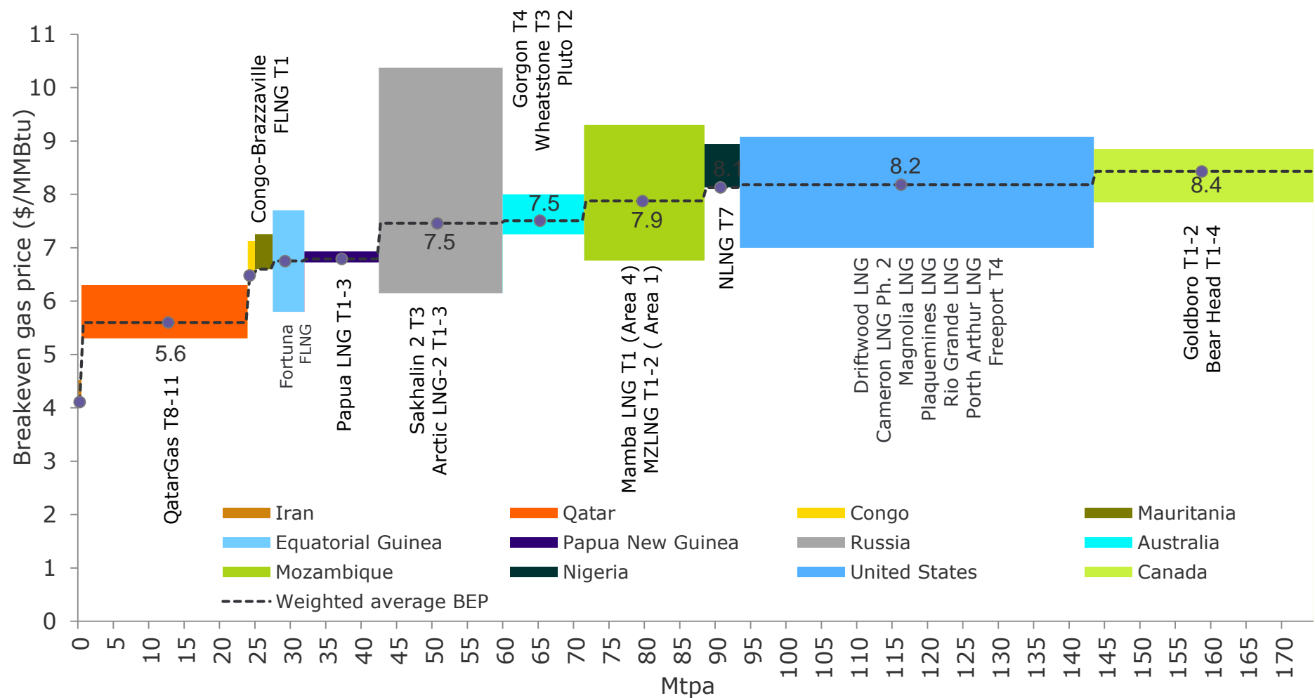
Volumes and breakeven prices for unsanctioned LNG projects by 2025
